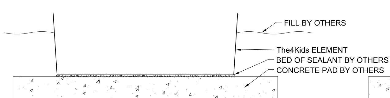
SEALANT BED
