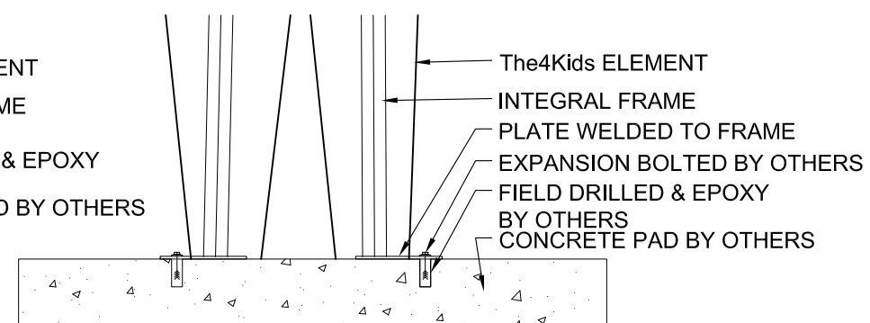
METAL TAB BOLTED TO CONCRETE PAD
