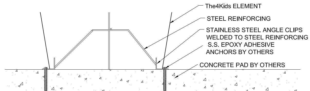
STAINLESS STEEL ANGLE CLIPS WITH ANCHORS
