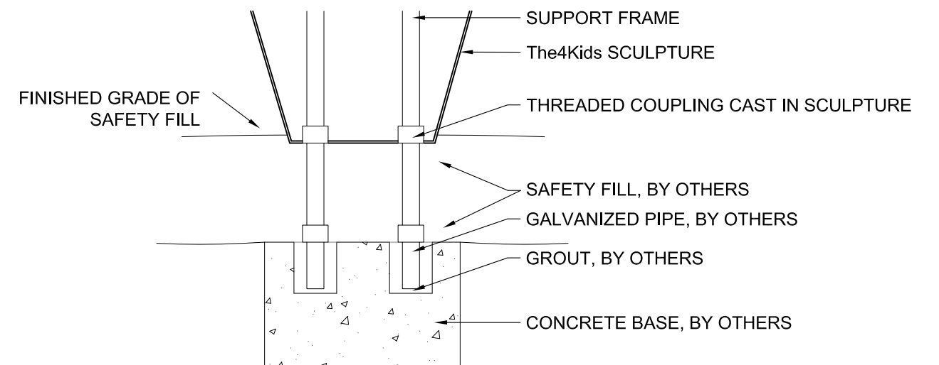
ADJUSTABLE METAL FOOTING IN CONCRETE PAD
