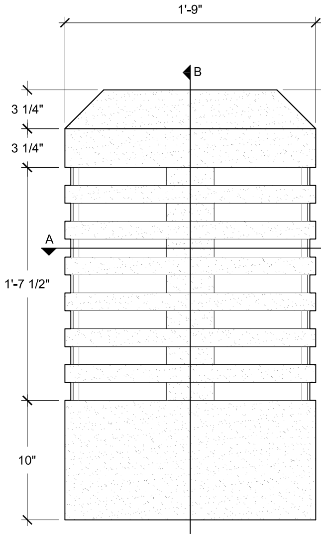
FRONT VIEW SCALE: 1 1/2" = 1'-0"
