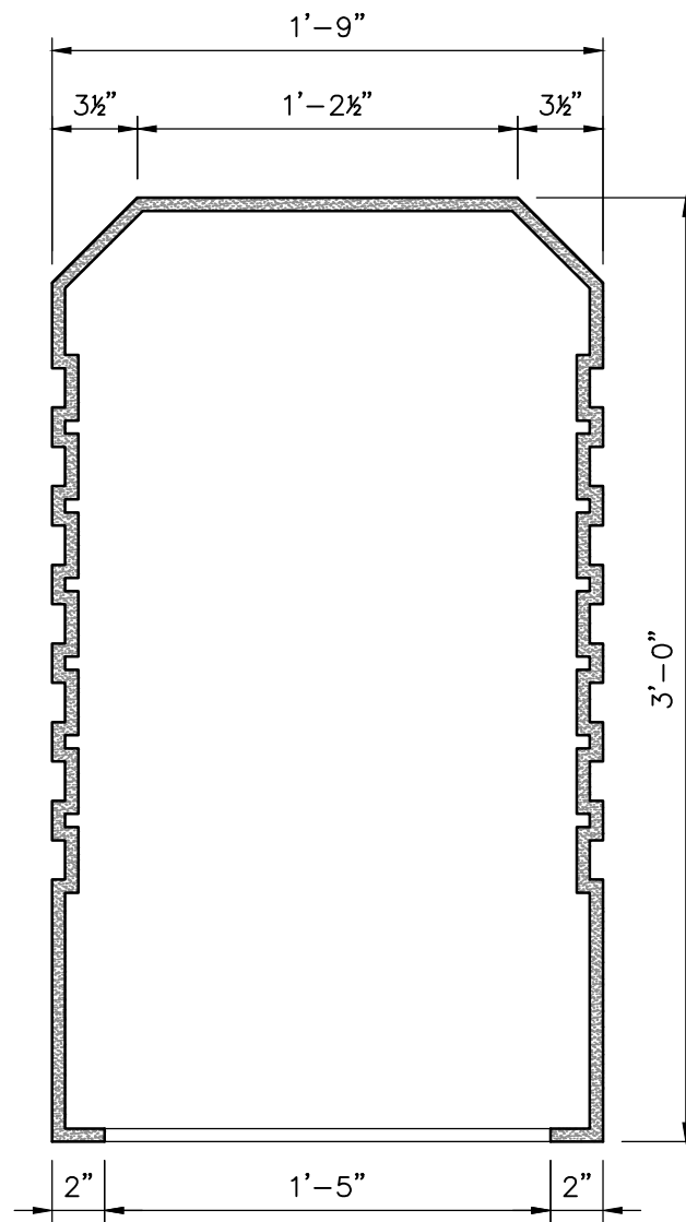
SECTION A
