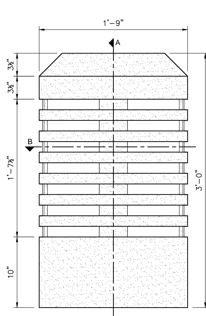
FRONT ELEVATION
