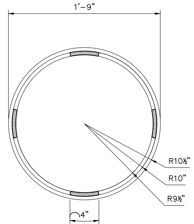
SECTION B
