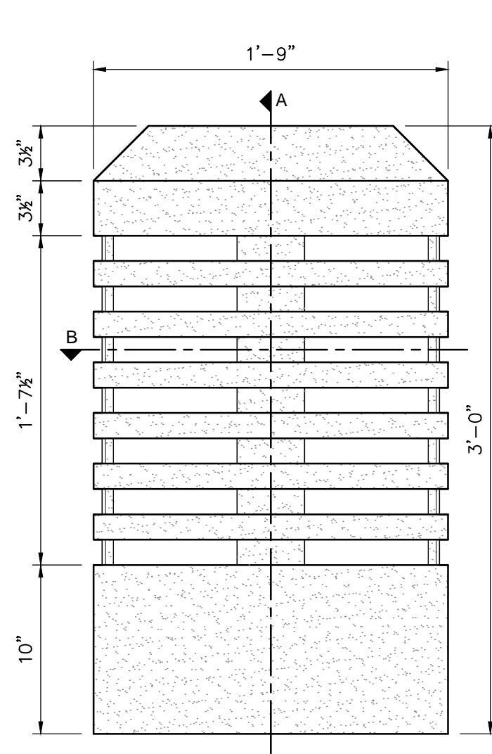
FRONT ELEVATION
