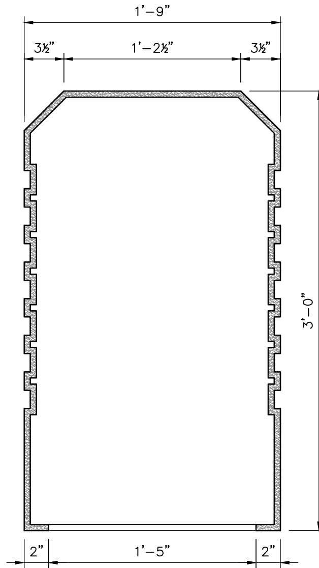
SECTION A
