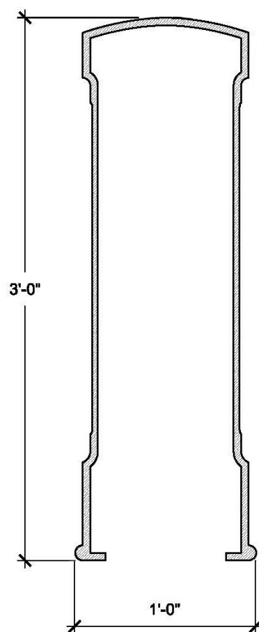
SECTION A
