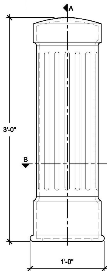
FRONT VIEW
