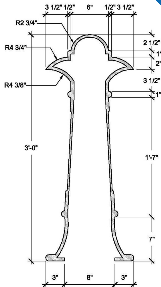
SECTION A
