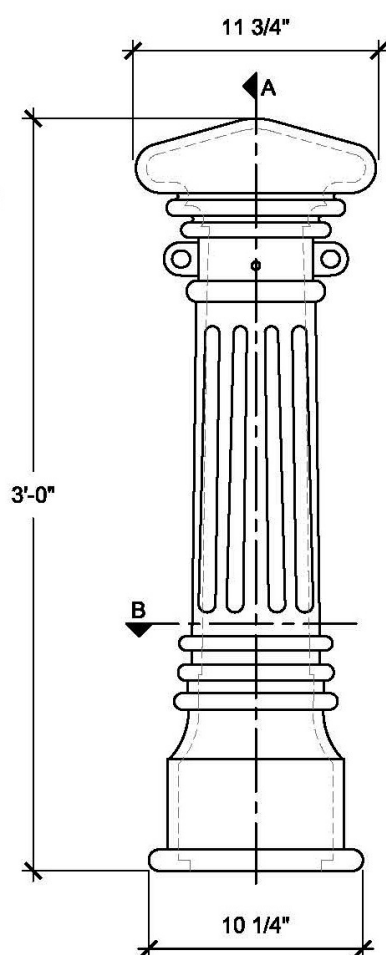
FRONT VIEW
