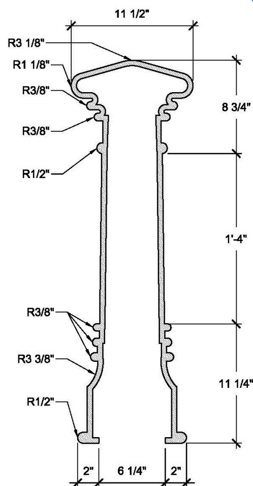
SECTION A
