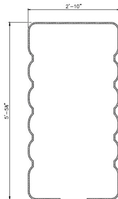
SECTION A
