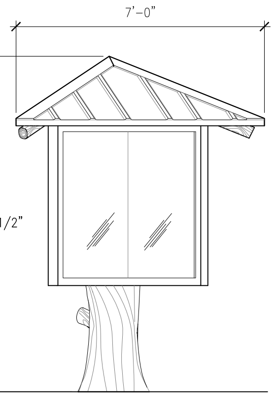
RIGHT-SIDE VIEW SCALE: \frac{3}{8}" = 1'-0"
