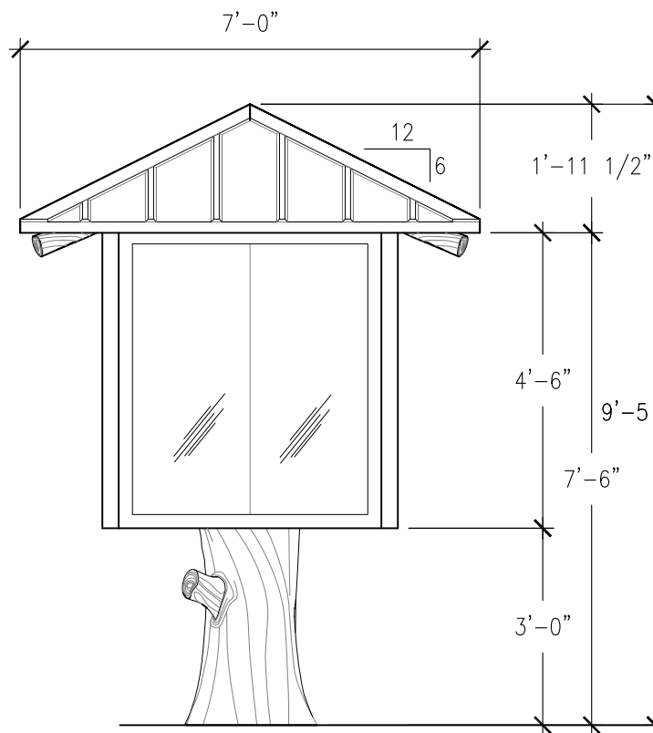
FRONT VIEW SCALE: \frac{3}{8}" = 1'-0"
