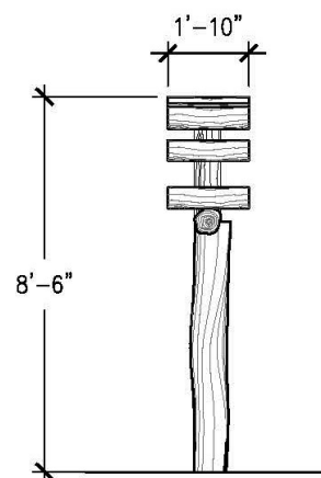
RIGHT-SIDE VIEW
