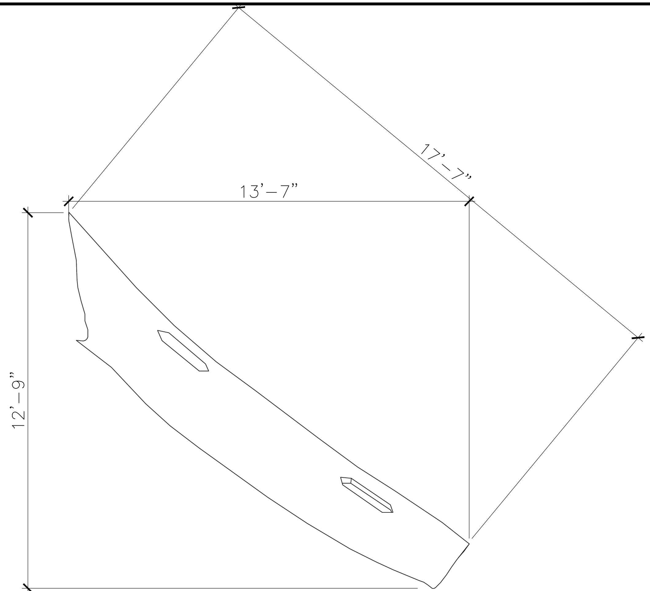
LEFT-SIDE VIEW
