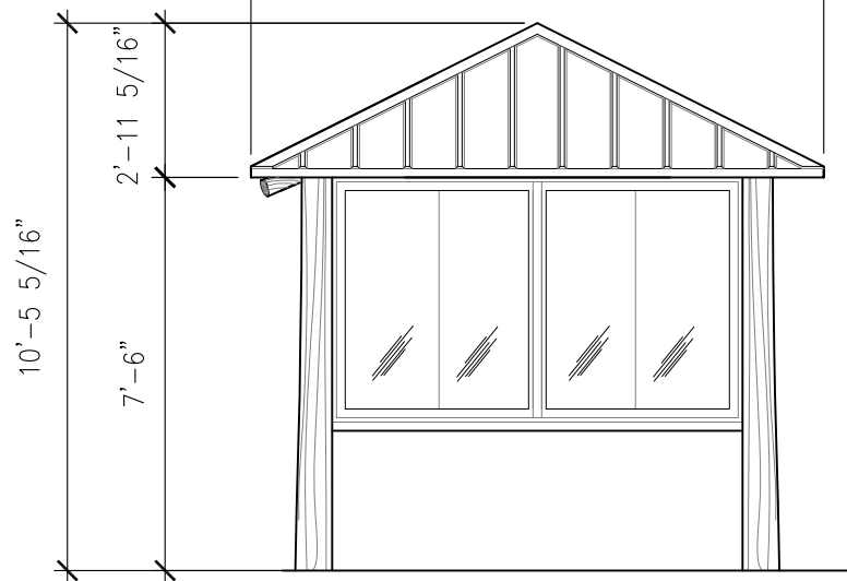
FRONT VIEW SCALE: 1/4" = 1'-0"
