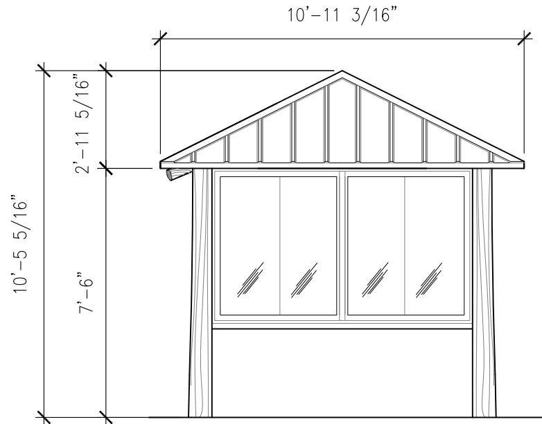
RIGHT-SIDE VIEW SCALE: 1/4" = 1'-0"
