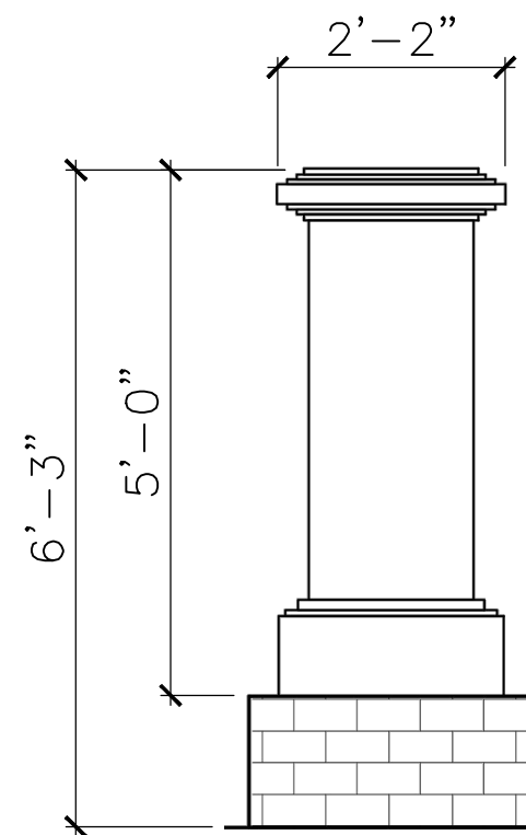
RIGHT-SIDE VIEW
