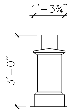
RIGHT-SIDE VIEW
