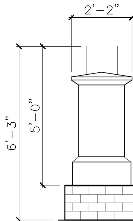
RIGHT-SIDE VIEW
