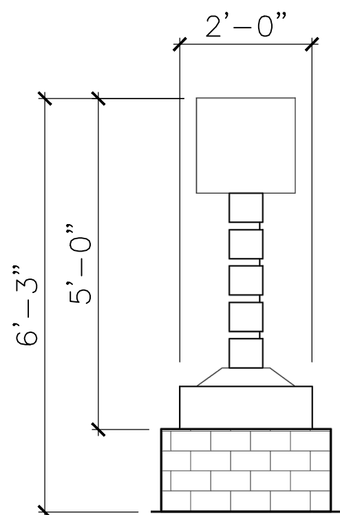
RIGHT-SIDE VIEW
