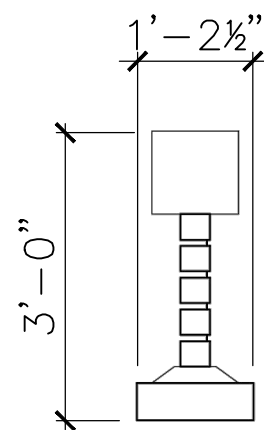
RIGHT-SIDE VIEW
