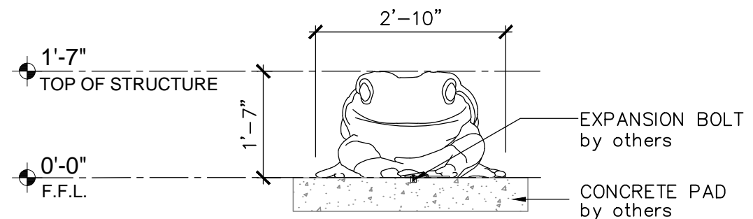
SIDE VIEW
