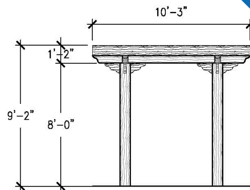
RIGHT-SIDE VIEW
